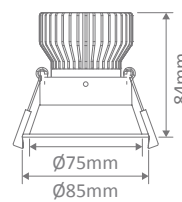
Cutout: Ø75-77mm
