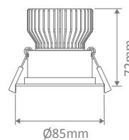
Cutout: Ø70-75mm
