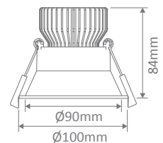
Cutout: Ø90-92mm
