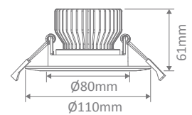
Cutout: Ø80-85mm
