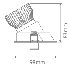
Cutout: Ø88-90mm
