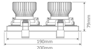
Cutout: L190mm x W100mm
