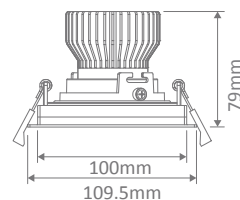
Cutout: L100mm x W100mm
