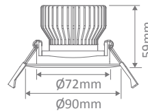
Cutout: Ø72-75mm
